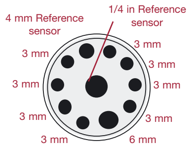
Multi-hole M03 (ATC-125 A/B)
